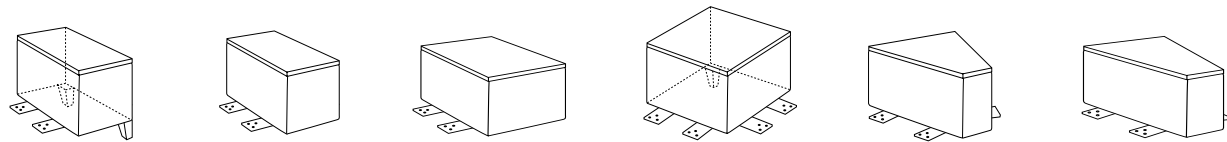
Ganging End Table with Two Legs: 378-1626EGT, 378-2226EGT Ganging End Table: 378-1626GT Ganging Lamp Table: 378-2226GT Ganging 90° Corner Table with One Leg: 378-9026CGT Ganging 45° Corner Table: 378-4526CGT Ganging 22.5° Corner Table: 378-2226CGT
